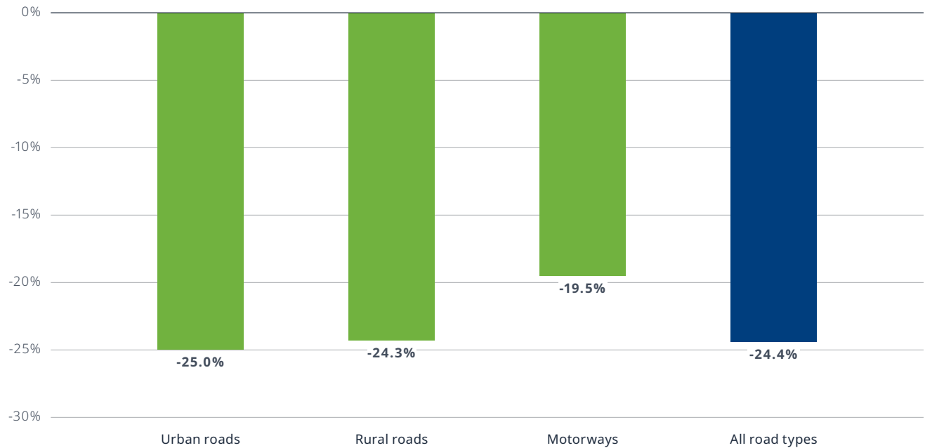
Figure 20: Evolution in road deaths by road type, 2023 compared to 2013
