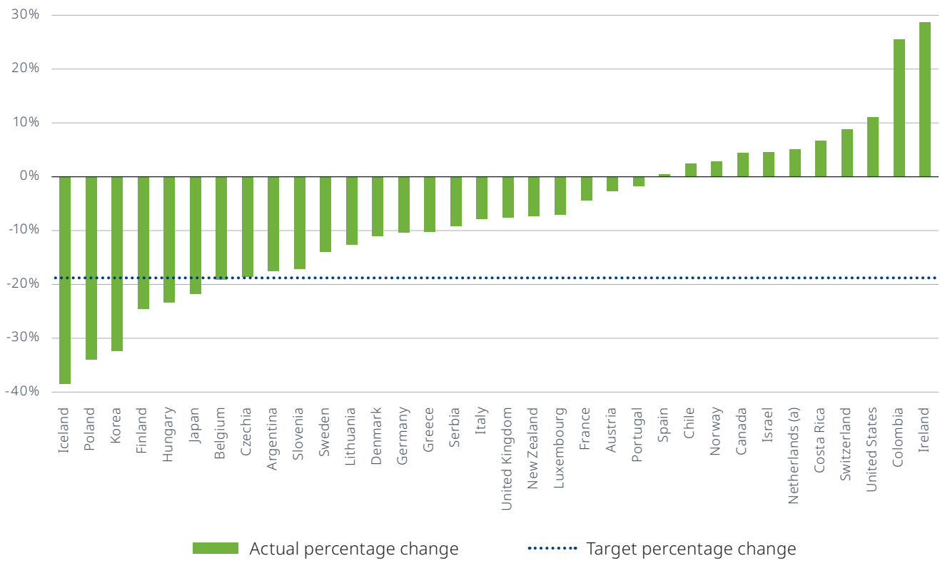
Figure 9: Percentage change in the number of road deaths, 2023 compared to the average 2017-19
