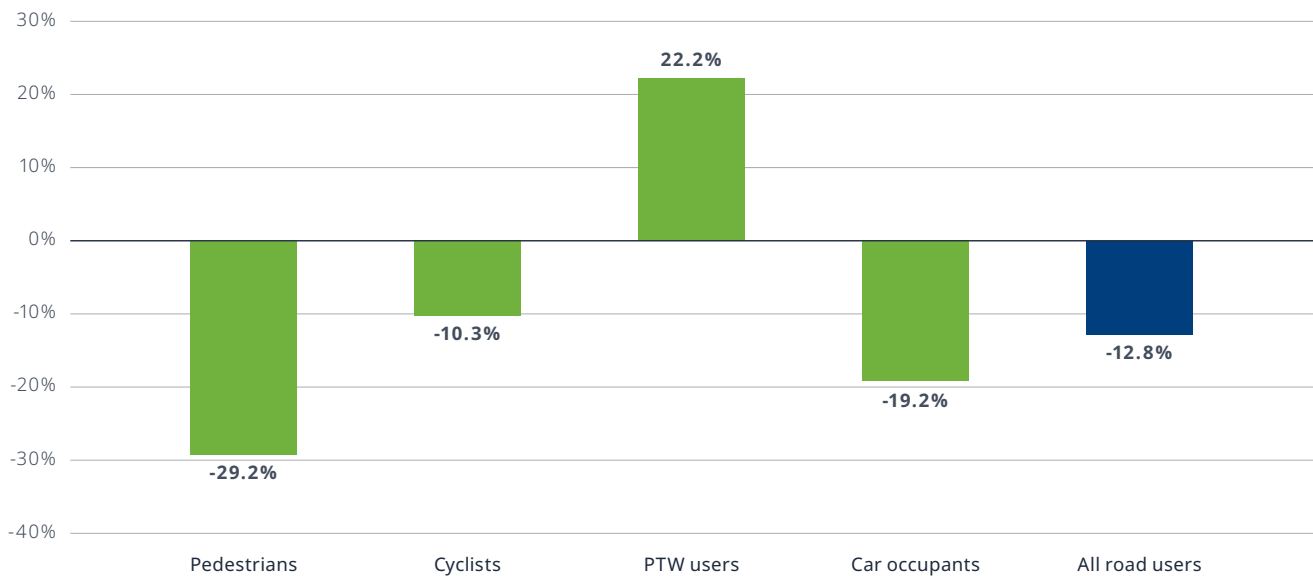
Figure 14: Evolution in road deaths by user category, 2023 compared to 2013
