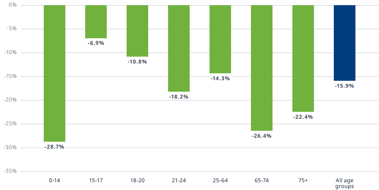
Figure 19: Evolution in road mortality rate by age group, 2023 compared to 2013
