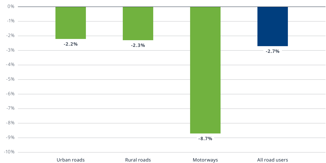
Figure 5: Evolution in road deaths by road type, 2023 compared to 2022
