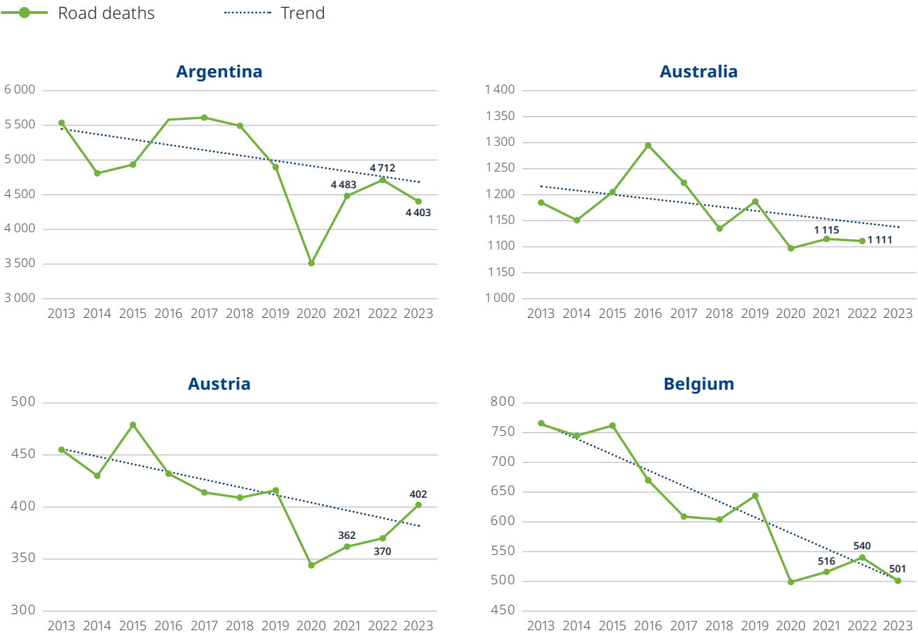
Figure 12: Road deaths compared to the linear trend since 2013 (excluding 2020 and 2021)
