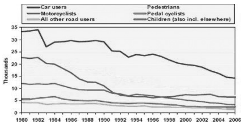
Figure 2: killed and serious injury for all type of transport
