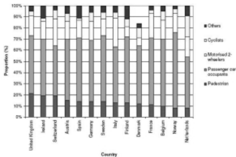
Figure 1: rate of fatalities over EU countries
