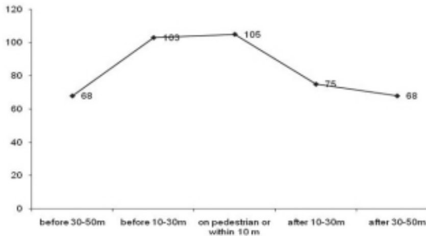
Figure 3: the most risky distance of pedestrian crossing facilities.
