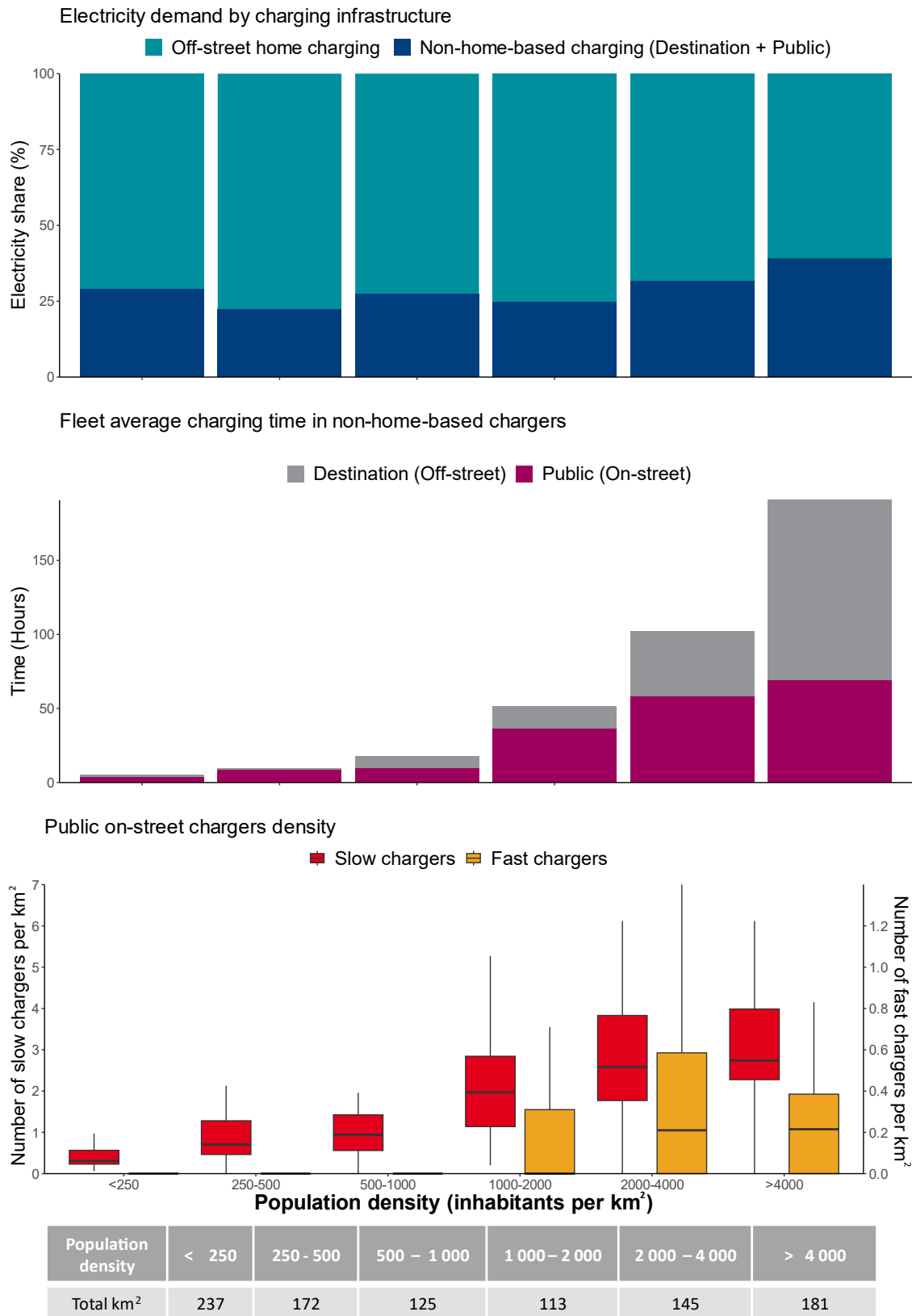
Figure 19. Public chargers in areas with different population densities (under high ambition)
