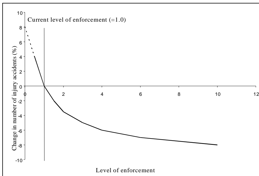
Figure 7. The relationship between level of enforcement and change in injury accidents (1= current level; 2 = twice as high, etc.)
